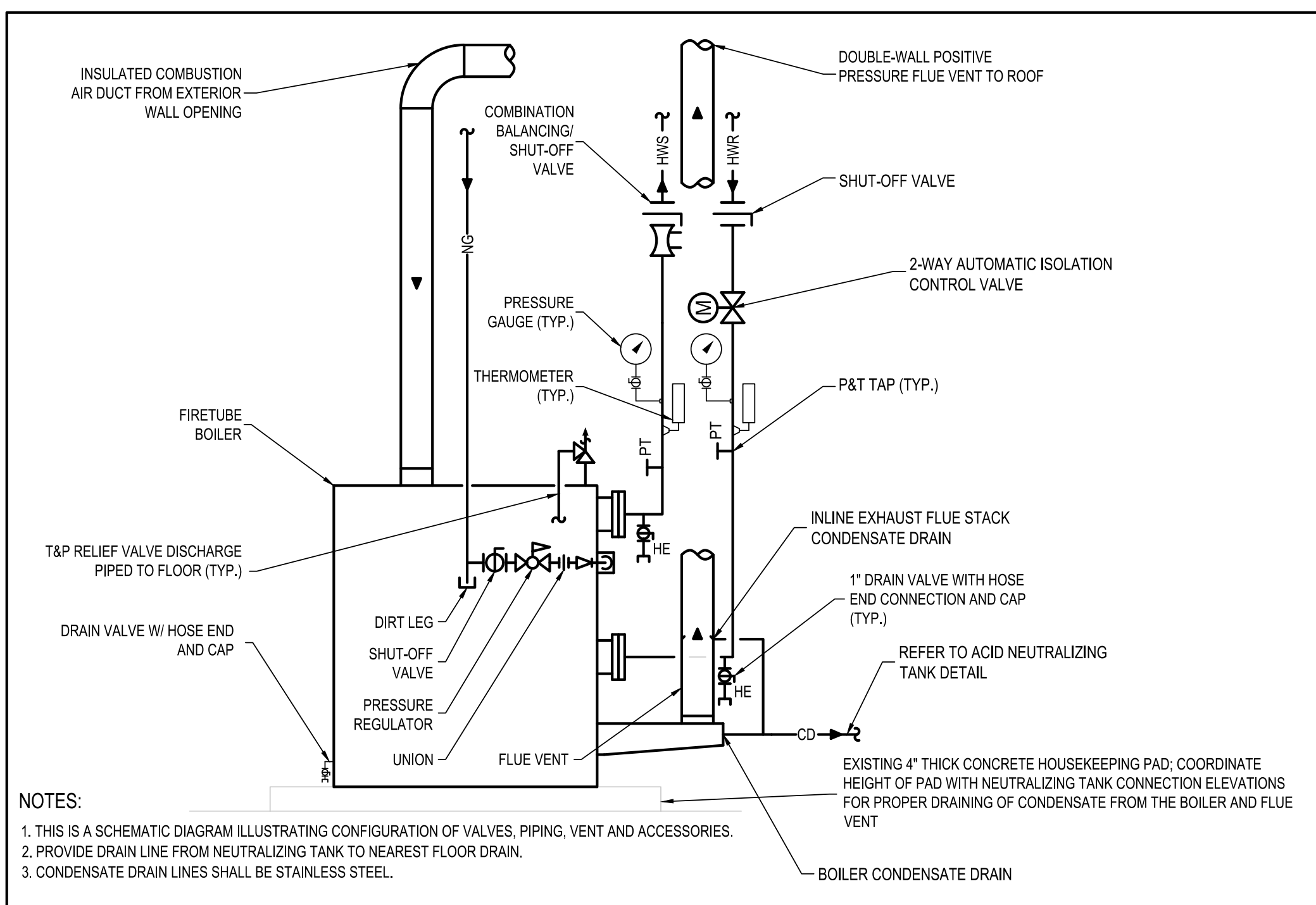
HOT WATER CONDENSING BOILER PIPING AND VENT CONNECTION DETAIL
