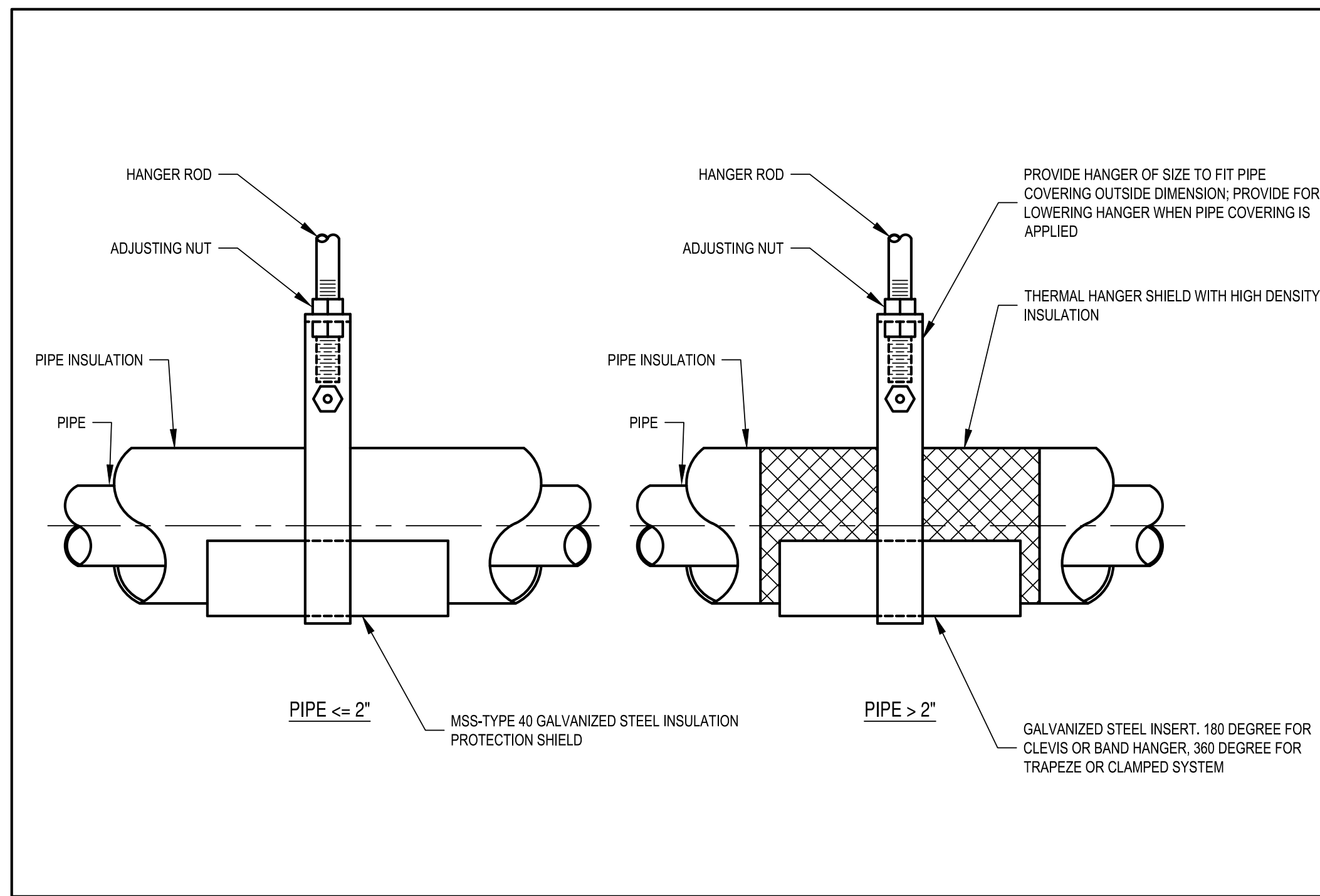
PIPE INSULATION SHIELD DETAIL
