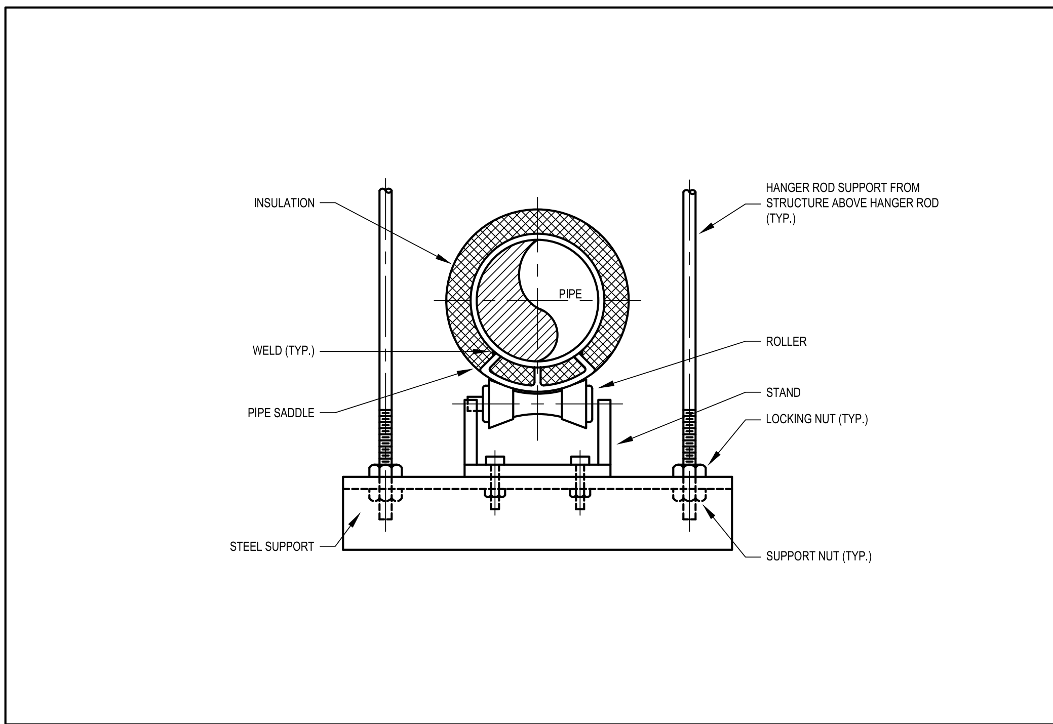
PIPE ROLLER HANGER DETAIL FOR HEATING HOT WATER PIPING
