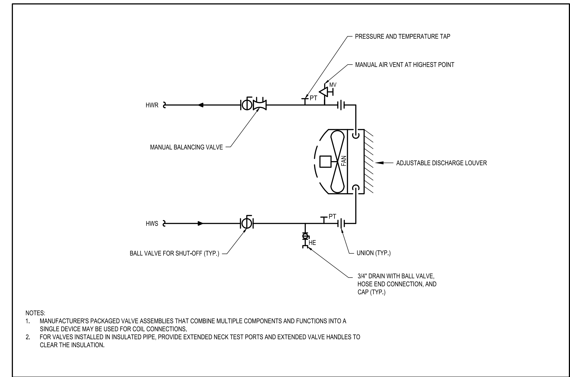
HOT WATER UNIT HEATER PIPING DETAIL - NO CONTROL VALVE
