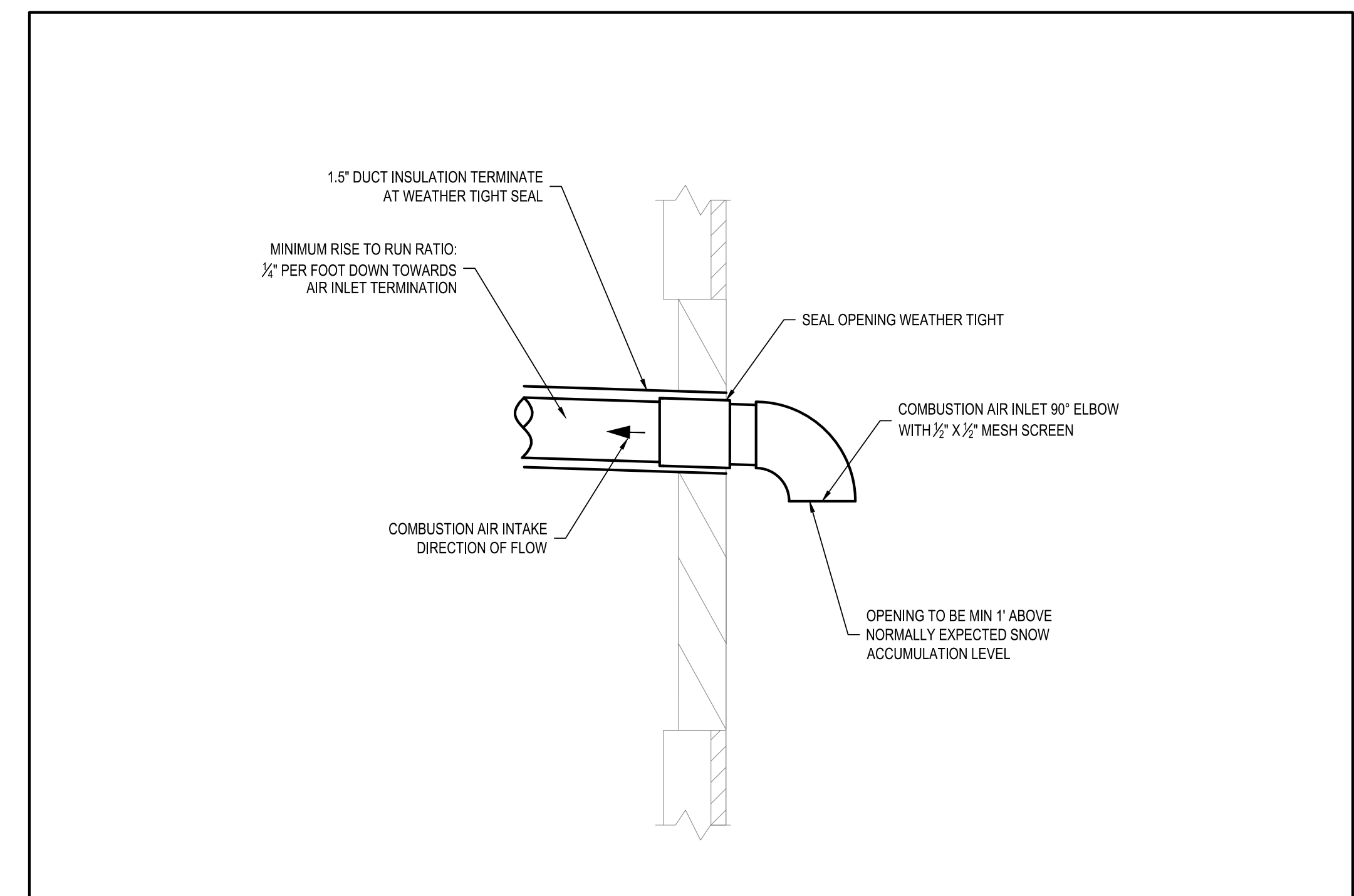
COMBUSTION INTAKE
