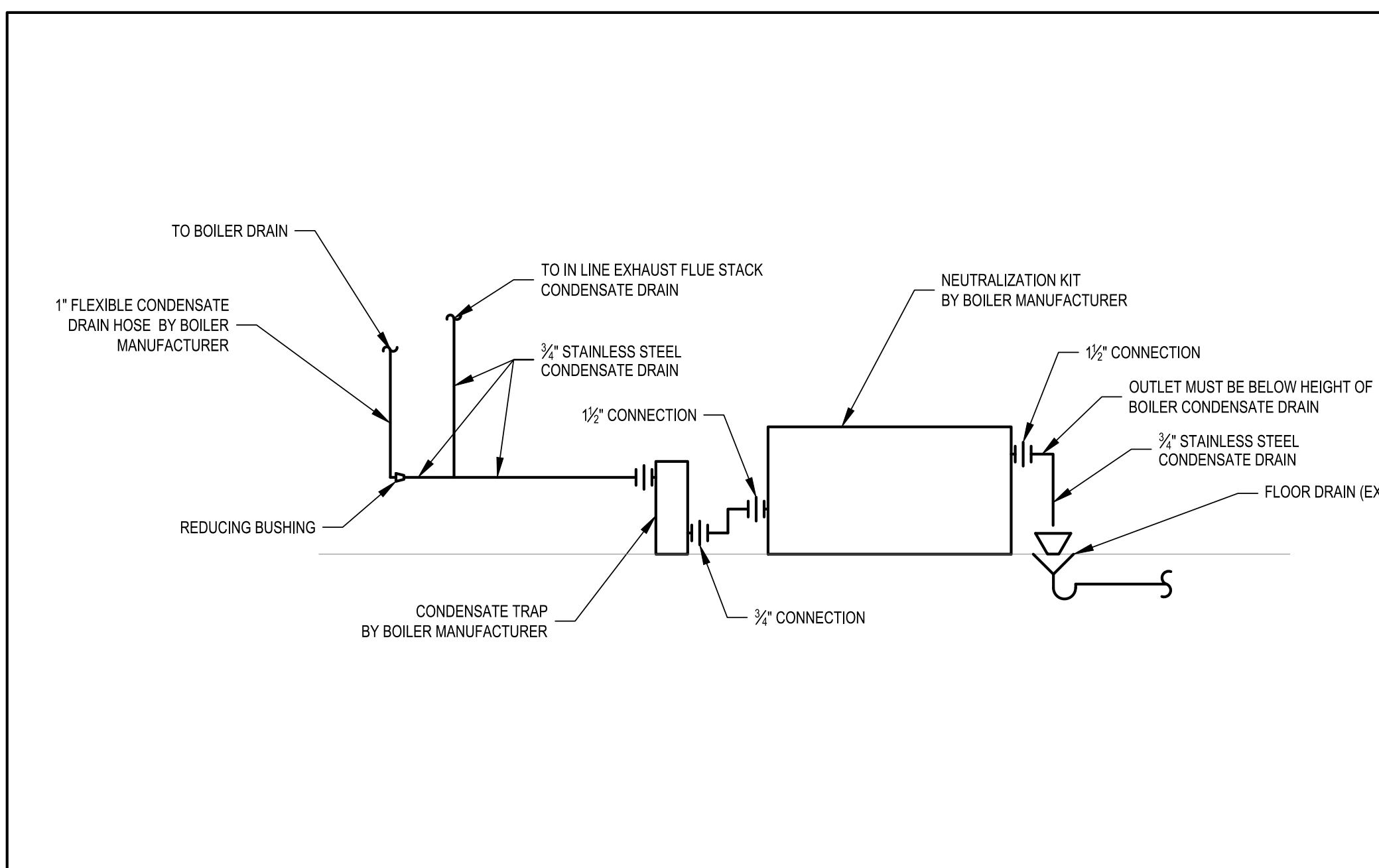
ACID NEUTRALIZING TANK DETAIL
